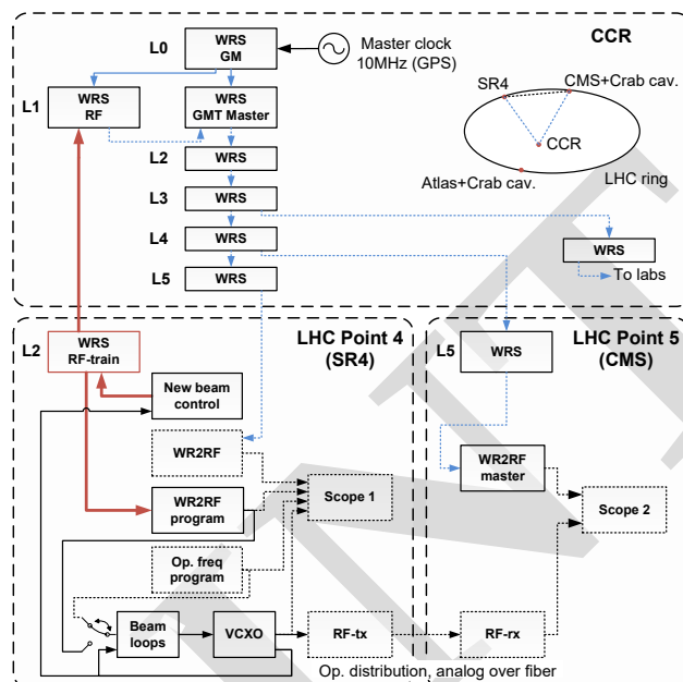
Figure 1: Test setup in the LHC. In red: the latency critical path, in blue: RF distribution over the general timing network. All dashed line equipment will be decommissioned after LS3.
