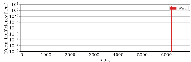
Figure 4: Betatron loss map without betatron collimator (TCSM.51932).
