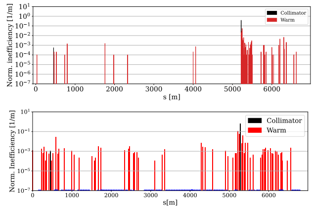
Figure 3: Simulated (upper) and experimental (lower) loss map with betatron collimator (TCSM.51932) at 5\sigma and off-momentum block (TIDP.11434) at nominal position.
