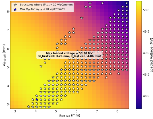
Figure 3: V_L for \langle a \rangle = 18 mm. White stars: W_{t,\text{tot}} < 10 ; blue star: optimal.
