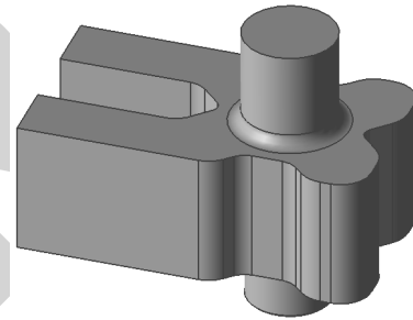
Figure 2: Geometry of the E-rotator with dual-polarized modes.
