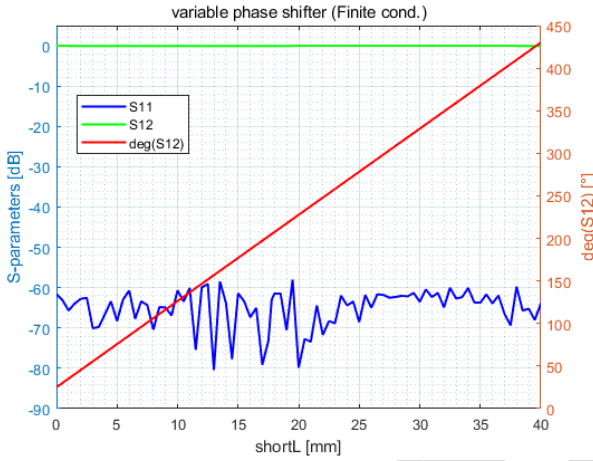
Figure 6: S-parameters of the variable phase shifter.
