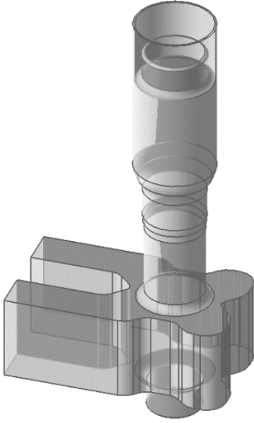
Figure 5: Geometry of the Variable phase shifter.
