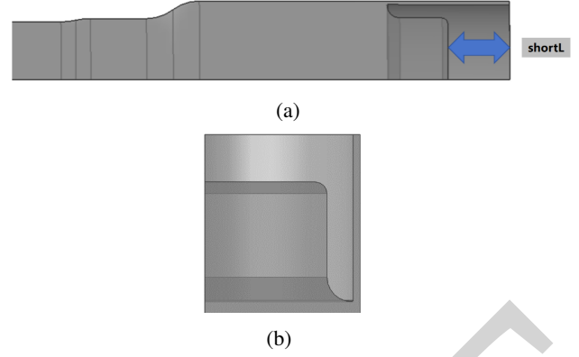
Figure 3: Movable short-circuited piston: (a) geometry (cut view) and (b) choke (cut view).
