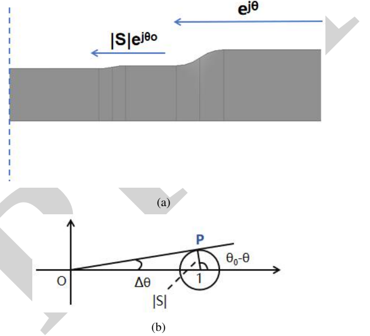
Figure 4: The transition section of the movable short-circuited piston: (a) schematic structure and (b) geometrical representation of phase variation.
