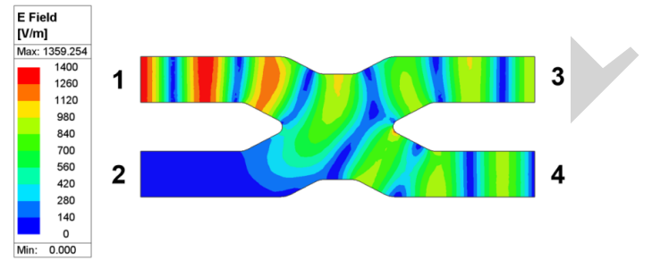
Figure 1: The electric field distribution for an E-hybrid.
