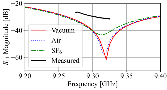
Figure 4: Simulated and measured reflected RF power S_{11} .
