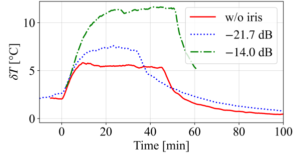
Figure 6: Temperature elevation during endurance tests.
