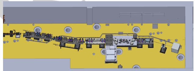
Figure 3: The transport line and the interaction section of the ELI-NP GBS.
