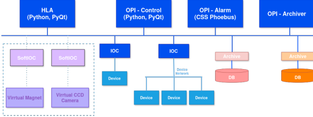
Figure 4: The architecture including EPICS Control, Archiving and Alarm for the ELI-GBS LINAC
