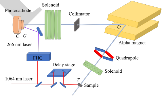
Figure 1: Schematic layout of the proposed MeV UED beamline based on a VHF gun and an \alpha -magnet compressor.
