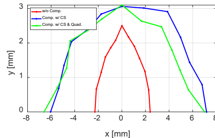
Figure 6: Dynamic apertures before and after compensation.
