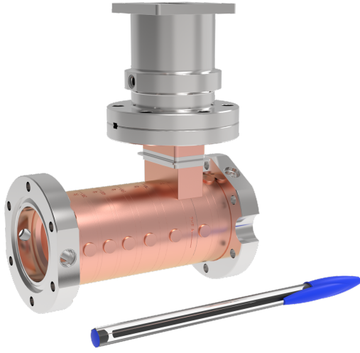
Figure 1: Accelerating structure mechanical design.
