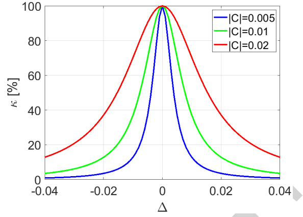
Figure 2: Variations of \kappa with \Delta at different skew quadrupole strengths.
