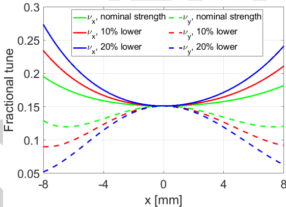
Figure 5: Horizontal ADTS for the lattice cases with different octupole strengths.
