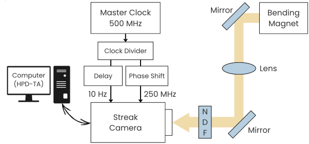
Figure 1: Block diagram of the streak camera measurement system.
