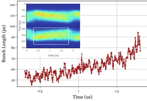
Figure 4: Measured bunch length distribution under SRF HC operation.
