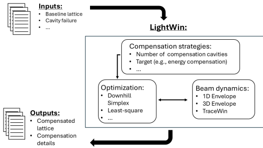
Figure 3: Simplified structure of LightWin.
