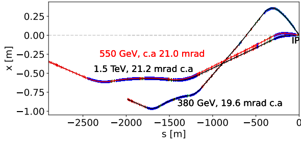
Figure 8: Layout of the 1.5 TeV, 550 GeV and 380 GeV lines aligned to the main linac and the interaction point, with crossing angles 21.2 mrad and 21.0 mrad respectively.
