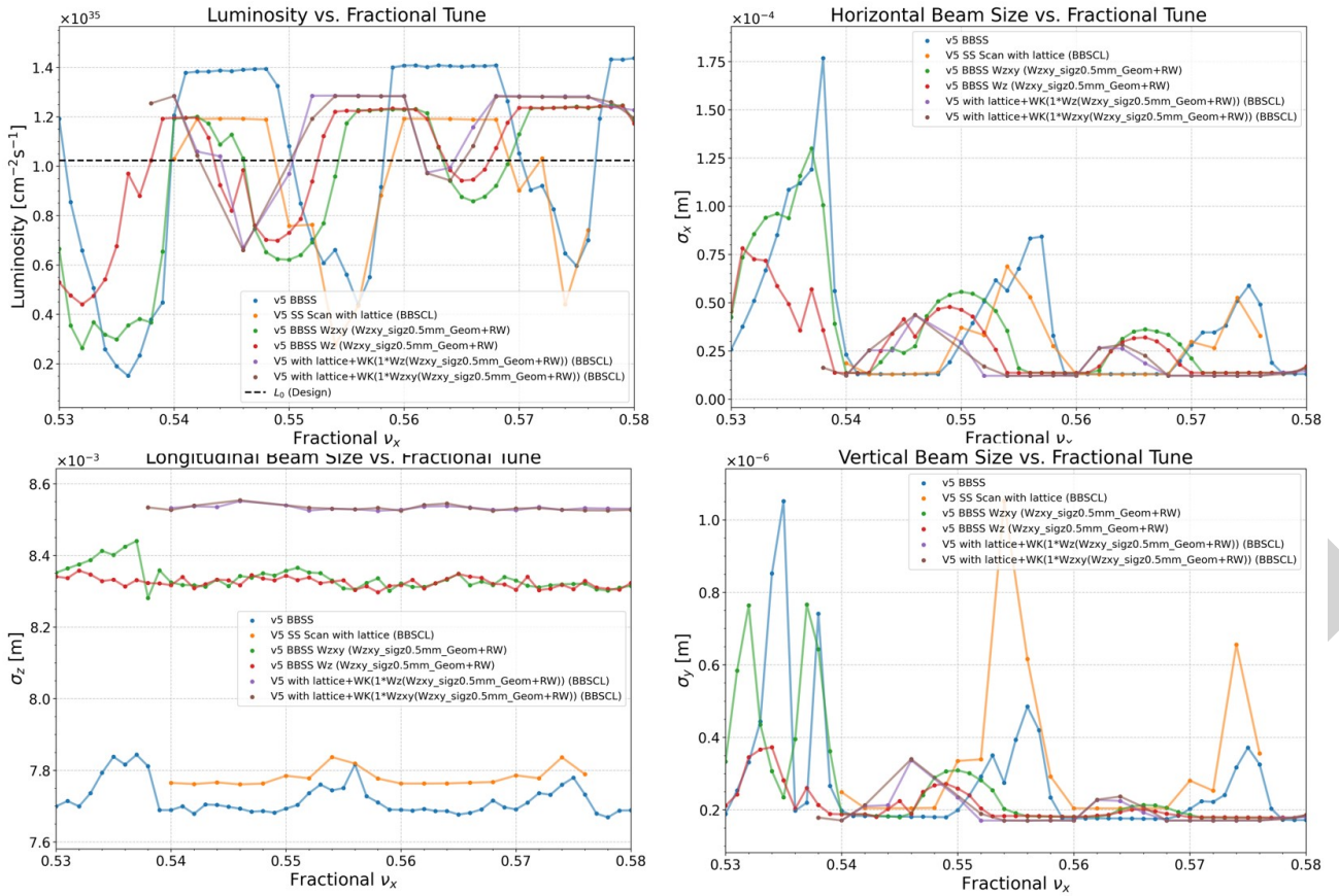
Figure 3: Simulated luminosity and beam sizes vs. \nu_x , comparing cases with W_z only and full 3D wakefields ( W_{x,y,z} ). The rightward translation of stopbands is clearly visible.
