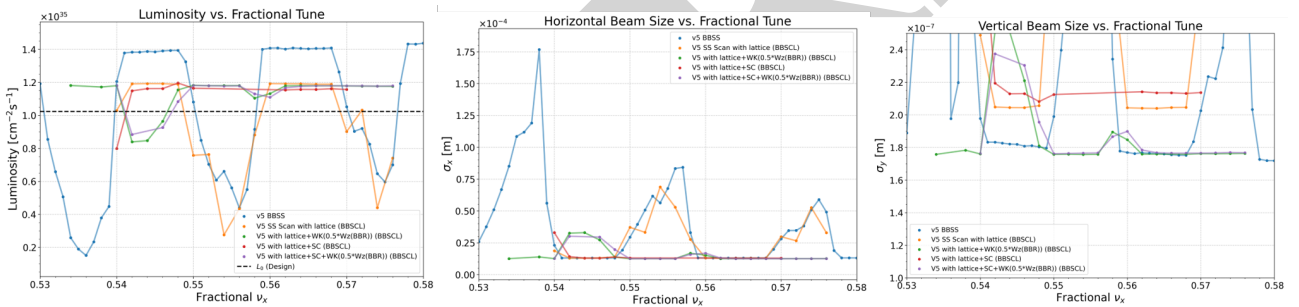
Figure 4: Impact of space charge (SC) effects. SC causes a global rightward shift of the resonance stopbands. Data within the severe XZI stopbands are smoothed due to catastrophic particle loss.
