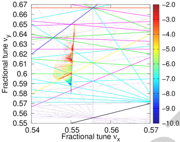
Figure 2: FMA for the STCF V5 lattice with and without beam-beam interactions.
