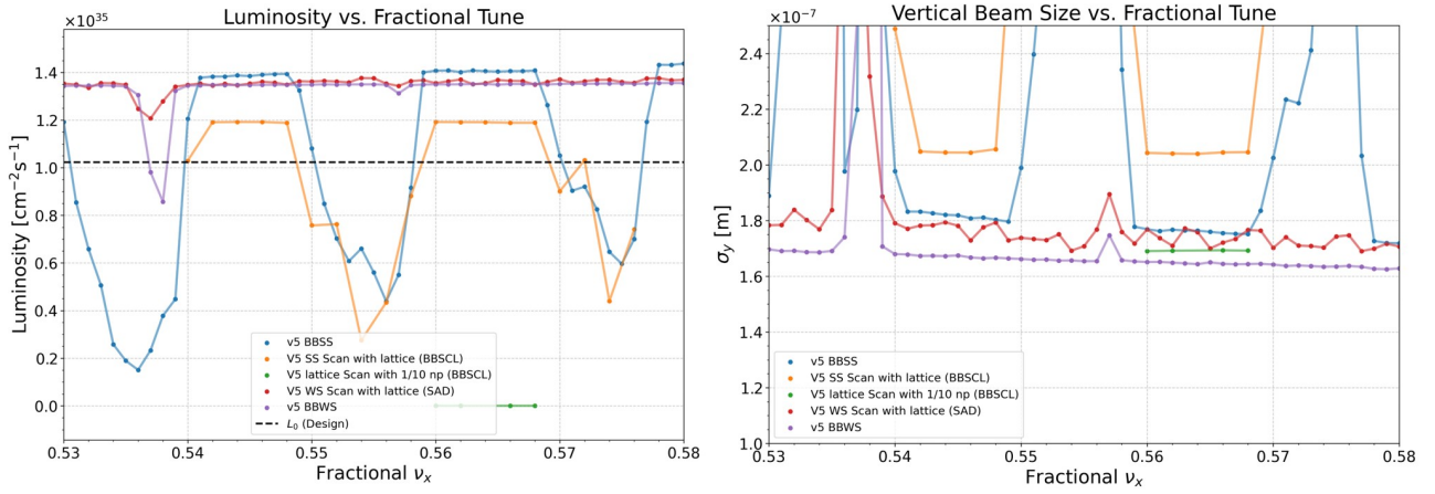
Figure 1: Luminosity and \sigma_y vs. \nu_x for various simulation models, illustrating the vertical beam size degradation driven by lattice nonlinearities.
