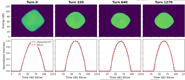
Figure 3: Longitudinal phase space tomographic reconstruction using real FCT measurement data from the XiPAF facility. The top row displays the reconstructed 2D phase space evolution, while the bottom row compares the 1D projected line density (dashed red) with the actual FCT measurements (solid grey).
