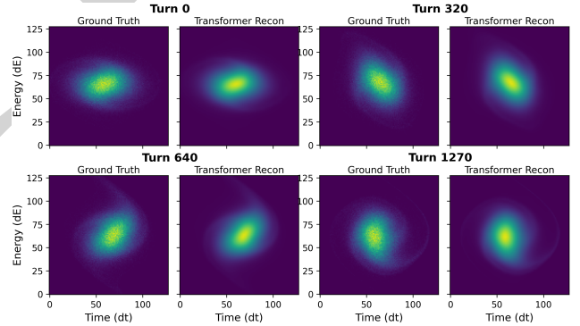
Figure 2: Snapshots of the longitudinal phase space evolution. For each specified turn, the ground truth (left) is compared with the Transformer reconstruction (right).
