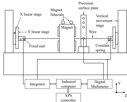
Figure 2: Layout of the measurement bench for the magnet fiducialization of the HALF.
