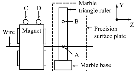
Figure 3: Schematic diagram of the precision surface plate and magnet fiducials. Two 0.5-inch target balls (A and B) are placed on the marble triangular ruler, while two 1.5-inch target balls (C and D) are positioned on the magnet fiducials.
