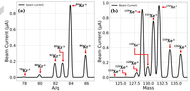
Figure 5: Isotope mass spectra of (a) Kr and (b) Xe beams extracted from the prototype FEBIAD.
