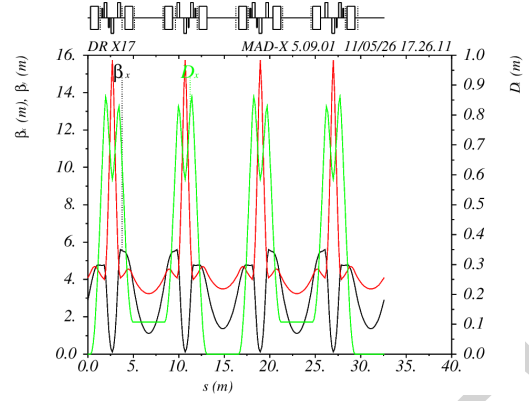
Figure 1: Optical functions of the extraction lattice. The plot shows \beta_x , \beta_y , and the horizontal dispersion D_x along the damping ring. The machine starts at the injection septum. The extraction septum is located after the second arc structure.
