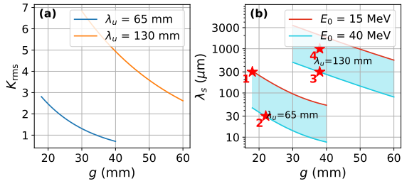
Figure 1: Undulator parameters as functions of the gap for the two APPLE-II undulators: (a) undulator parameter K , and (b) FEL wavelength \lambda_s for beam energies from 15 MeV to 40 MeV.
