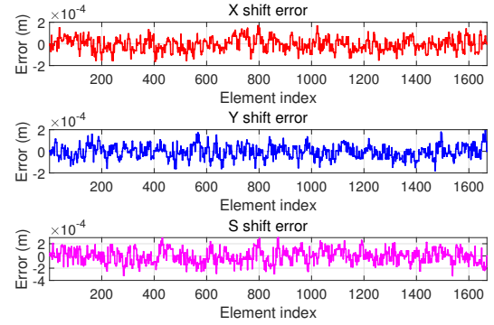
Figure 2: Shift errors of the storage ring.
