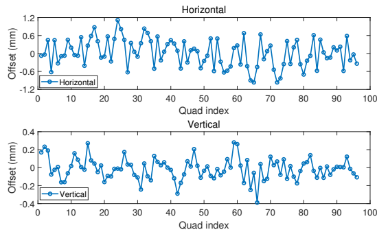
Figure 6: BBA measurement results.
