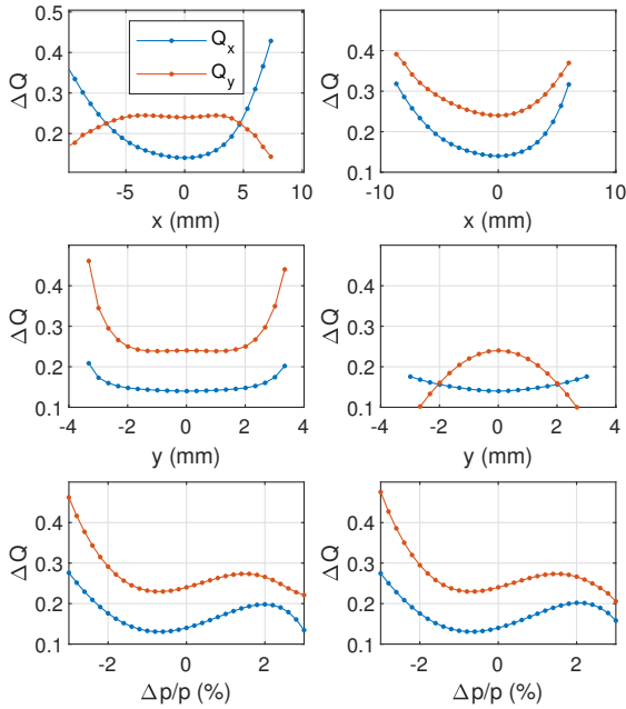
Figure 5: Comparison of tune-shifts with amplitude and energy. Left column: ideal hard-edge model. Right column: including crosstalk.
