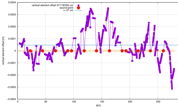
Figure 3: Vertical girder fits after initial alignment (blue squares) with respect to the alignment network ranging from -300\text{ }\mu\text{m} to +350\text{ }\mu\text{m} . The location of the source points in the straight sections is indicated by red dots.
