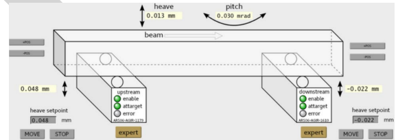
Figure 5: Controls interface for the remote vertical girder alignment. Motors and encoders provide a 1\text{ }\mu\text{m} positioning resolution of the girder feet. Corresponding heave and pitch values are calculated.
