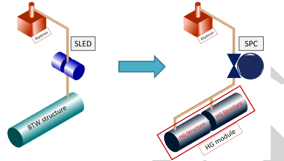
Figure 2: FERMI linac upgrade plan to replace BTWs and SLEDs with the HG modules and SPC.
