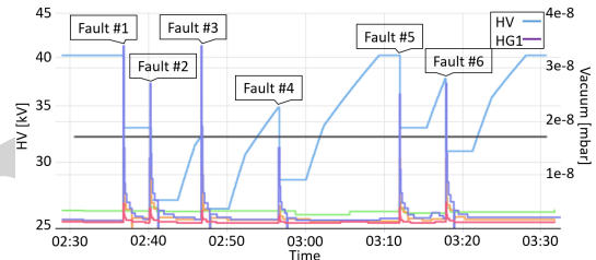
Figure 12: Example of long fault at the HG1.
