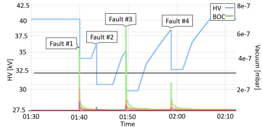
Figure 11: Example of the long fault in the BOC region.
