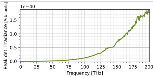
Figure 2: Peak detector irradiance vs. frequency from simulations.
