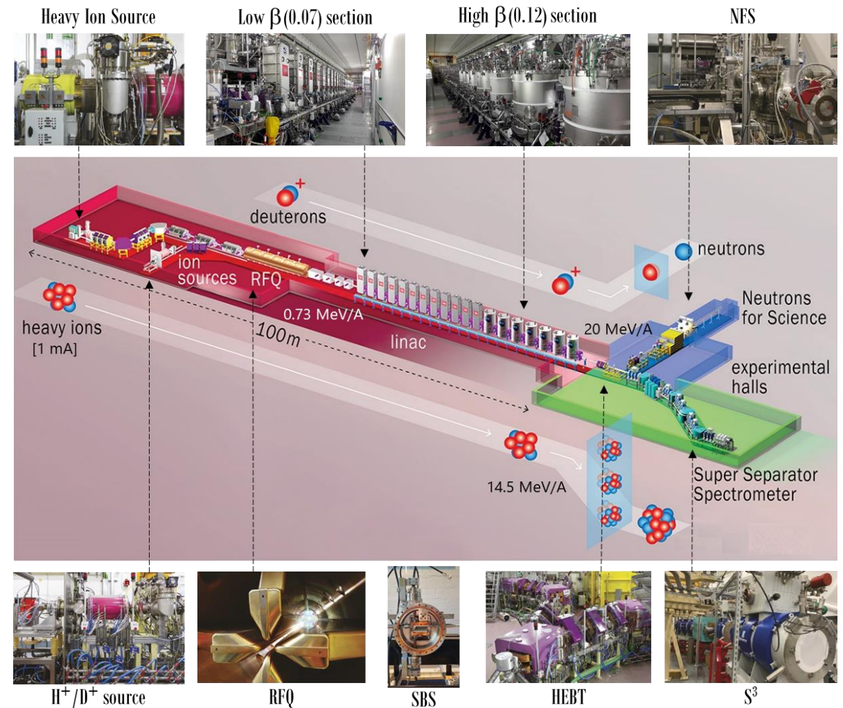
SPIRAL2 SC linac — from ion sources to NFS and S3 experimental rooms (Source: GANIL/SPIRAL2)
