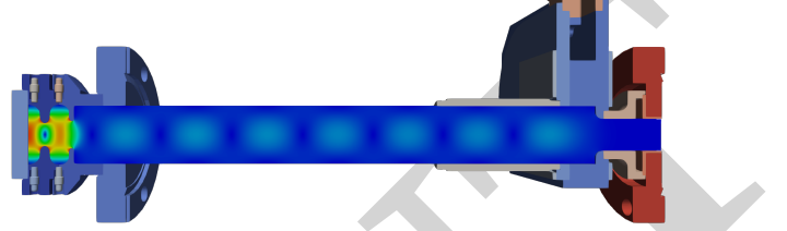
Figure 1: Cut-away view of the relative spacing between the CUPID photogun, the connecting waveguide, and the TM 10 mode launcher, with superimposed \pi -mode field map. The relatively long waveguide connecting both components is a design choice to accommodate the physical size of a solenoid designed for bright beam generation. Extended waveguide and solenoid are not shown in this view.
