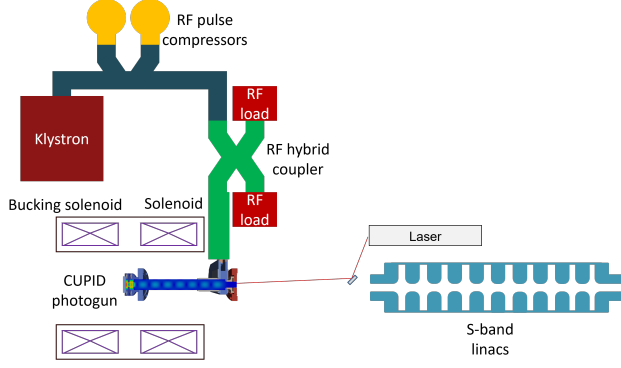
Figure 2: Rf pulses generated from the klystron (red box) is compressed by rf pulse compressors (yellow circles) into high power short rf pulses, which then sent to the rf hybrid coupler. Rf pulses are split into two output ports, where one of them is connected to our CUPID photogun. The other output port is connected to a rf load. Since more than 95 % of rf power will be reflected from CUPID photogun, another rf load is connected to the last port of the hybrid coupler to prevent reflected pulses from damaging the klystron. CUPID photogun is enclosed by a superconducting solenoid and connected to downstream S-band linacs.
