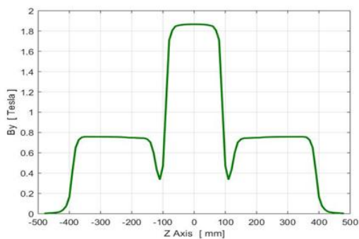
Figure 4: LG dipole magnet profile.
