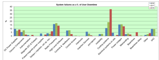
Figure 2: System failures as percentage of user downtime for 2016, 2017 and 2018.
