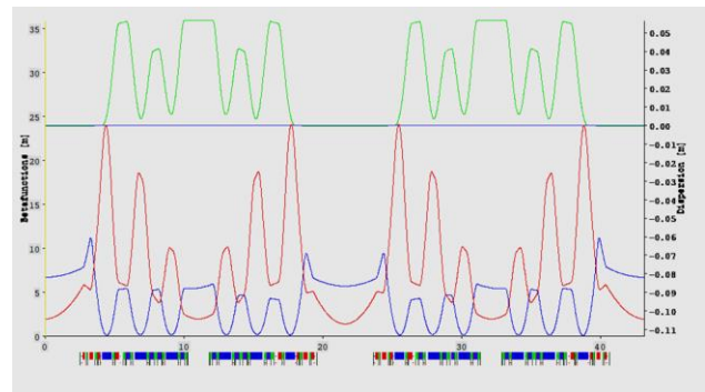
Figure 3: The S6BA_E lattice with LG dipoles (2-4 from left at each achromat) and reverse bend quadrupole / dipoles.
